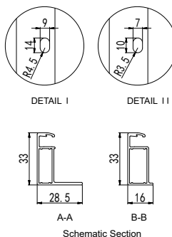
Schematic Section
