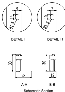
Schematic Section
