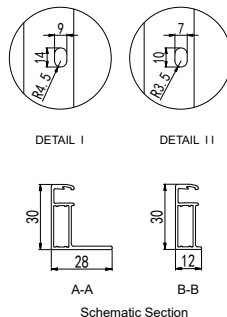
Schematic Section
