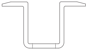
Figure 16: Detail of a clamp
