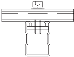
Figure 14: Tighten clamp
