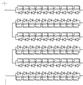
Figure 7-1: Electrical circuitry of cell strings and bypass diodes
