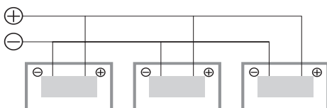
Figure 5: Electrical diagrams of series and parallel wiring
