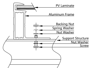
Figure 11: Detail of a bolt installation attachment
