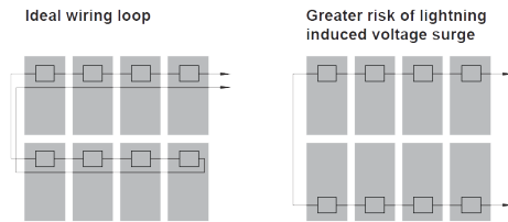
Figure 4: Wire loop design recommendation
