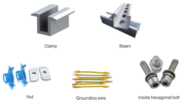
Figure 11: Installation accessories
