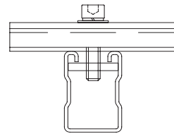
Figure 14: Tighten clamp
