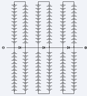
Figure 7: Electrical circuitry of cell strings and bypass diodes
