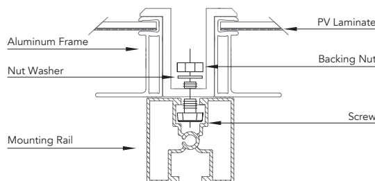
Figure 13: Detail of a top-down clamp installation attachment
