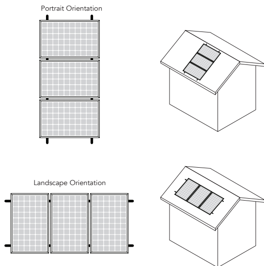
Figure 10: Landscape and portrait installation
