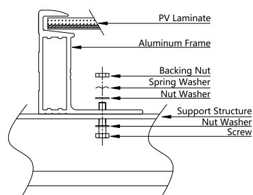
Figure 11: Detail of a bolt installation attachment
