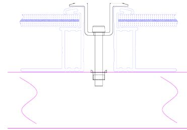
Figure 13: Tighten clamp
