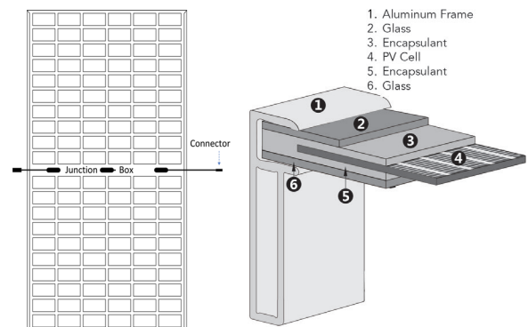
Figure 1: Module components and cross-section of the laminated assembly
