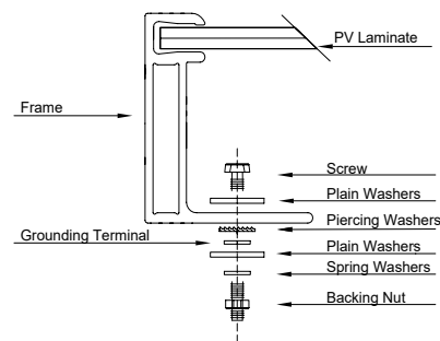
Figure 9: Grounding screw assembly detail
