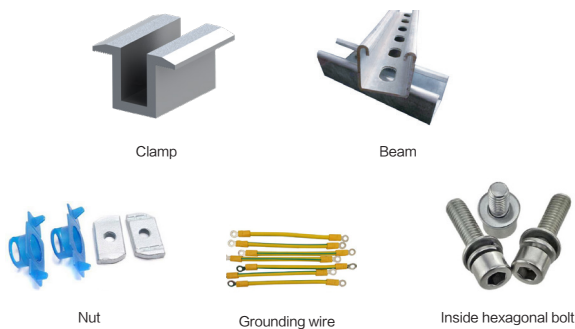
Figure 11: Installation accessories
