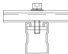
Figure 14: Tighten clamp
