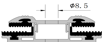
Figure 11: Detail of a clamp
