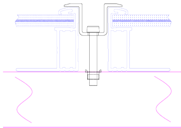
Figure 19: Tighten clamp
