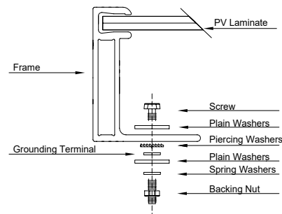
Figure 10: Grounding screw assembly detail
