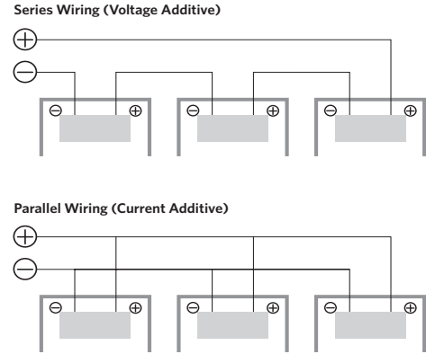
Figure 6: Electrical diagrams of series and parallel wiring
