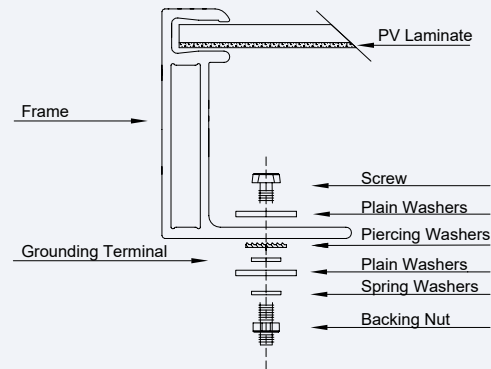
Figure 9: Grounding screw assembly detail
