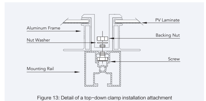
Figure 13: Detail of a top-down clamp installation attachment
